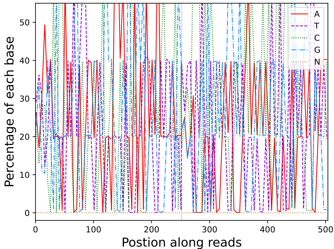
Base percentage along reads (R20211)
